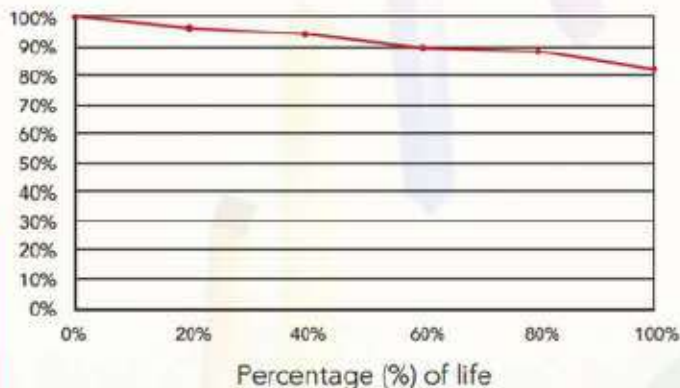
Lumen Maintenance (%)
